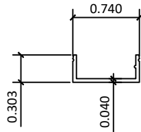
15 5500-09 - HEAD SCREW COVER
