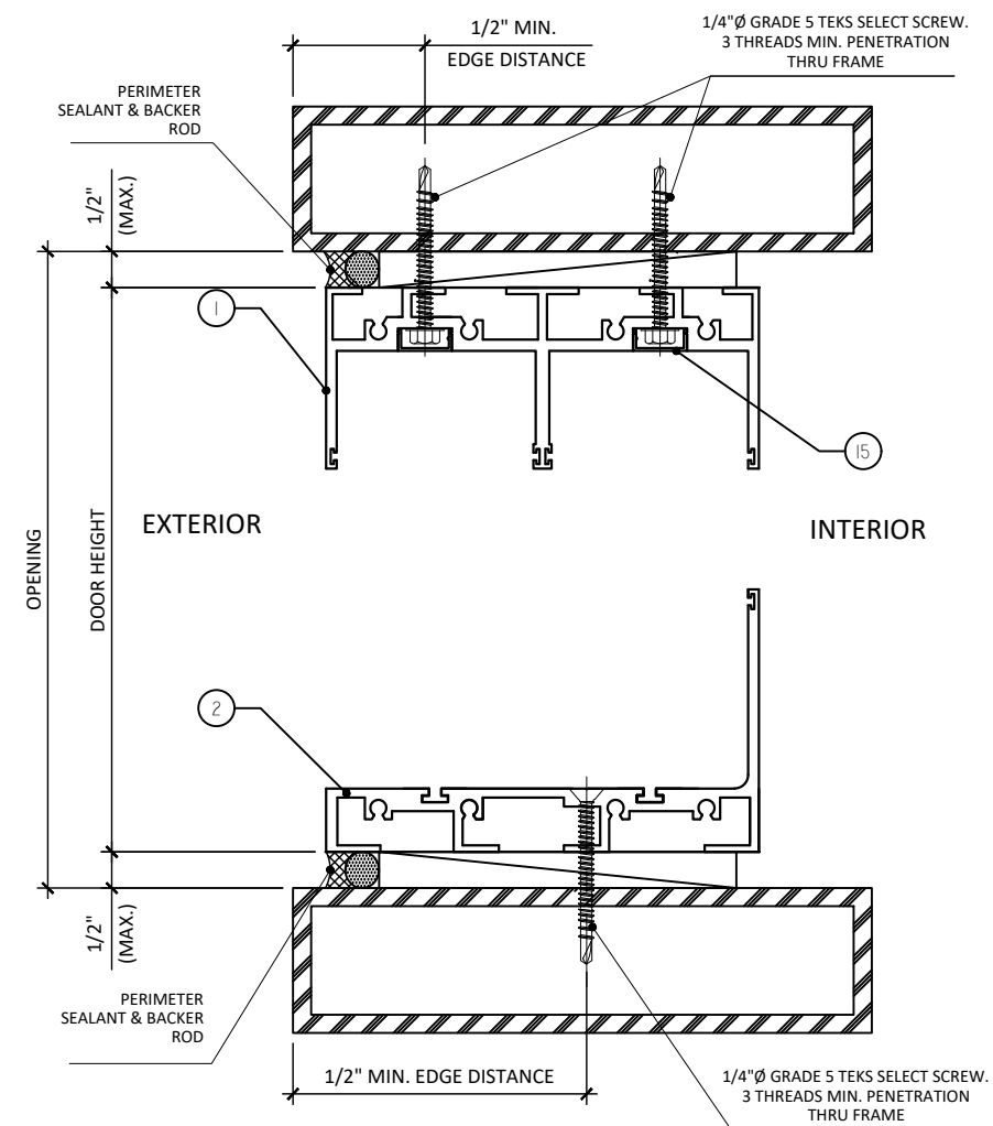
ALUMINUM TUBE HEAD & SILL
