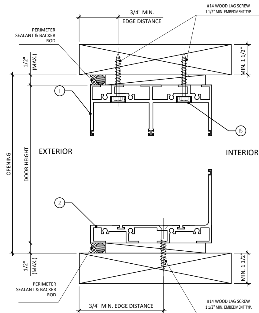
PT WOOD BUCK HEAD & SILL
