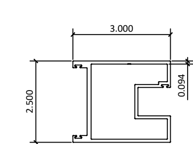
8 2800-13 – FIXED STYLE
