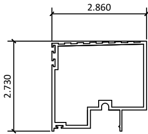
14 2800-24 - THRESHOLD
