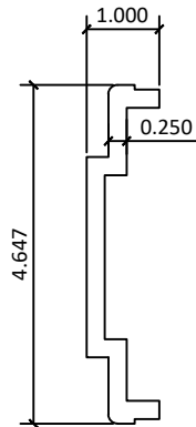
21 3000-14 - MALE & FEMALE REINFORCEMENT
