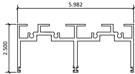
1 2800-02 – HEAD
