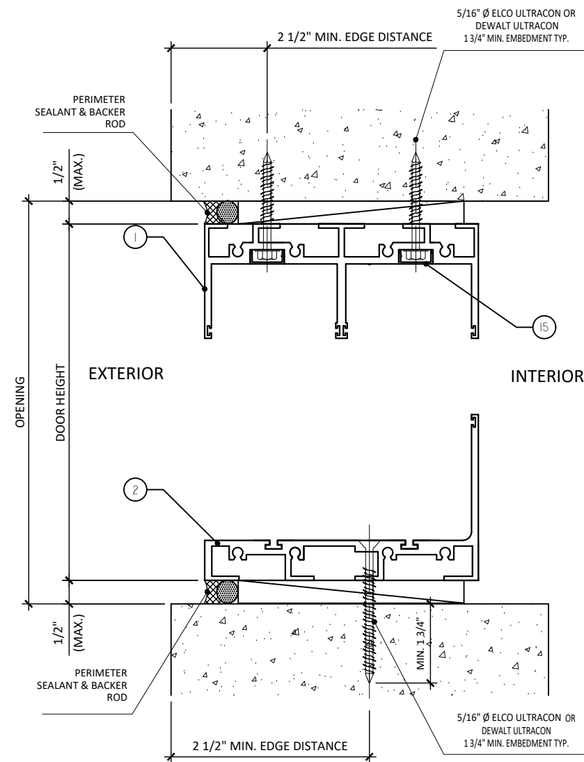
MASONRY HEAD & SILL
