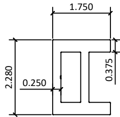
16 2800-23 - REINFORCING
