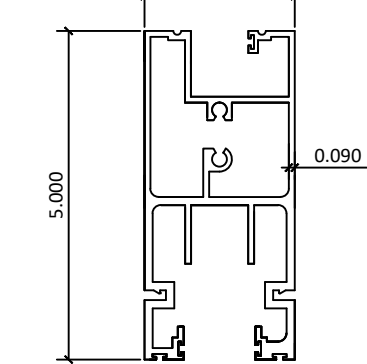
4 2800-09 – MOVING PANEL
