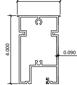
3 2800-08 – TOP PANEL
