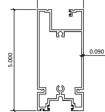
5 2800-19 – BOTTOM FIXED PANEL
