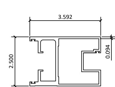
7 2800-10 – MOVING PANEL
