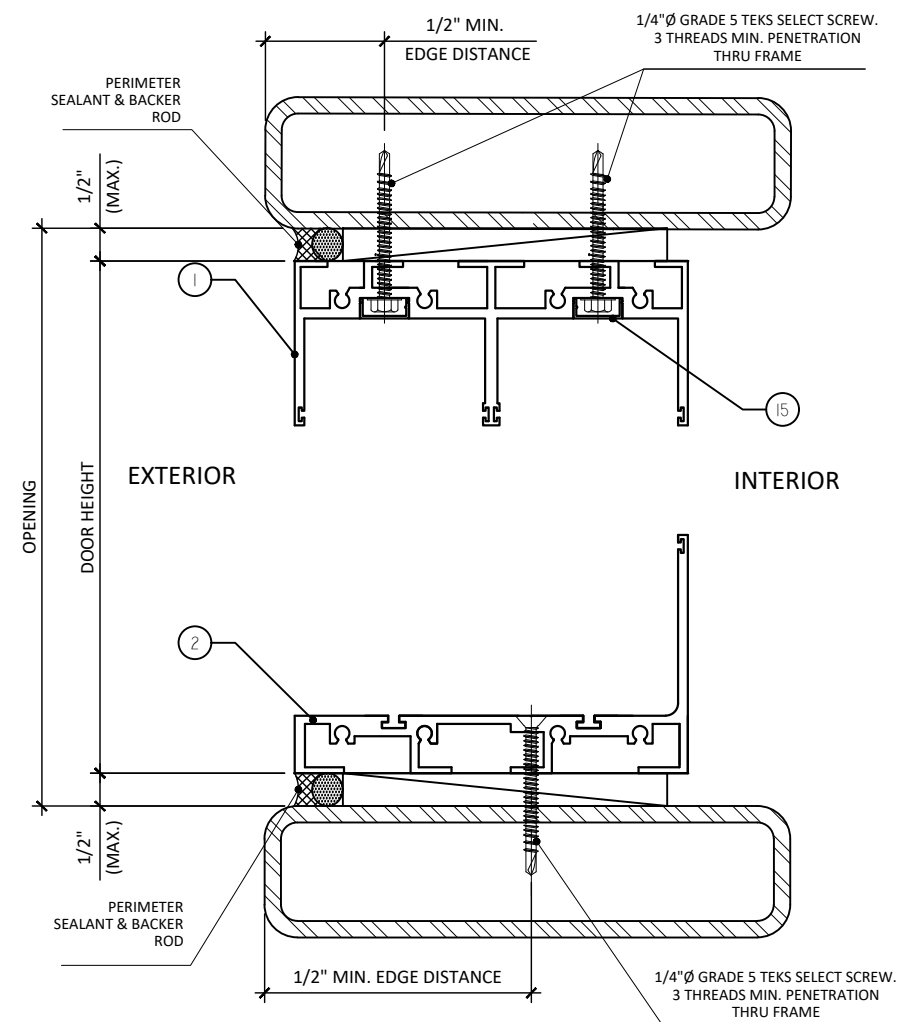
STEEL TUBE HEAD & SILL
