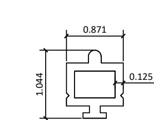
13 2800-05 – SILL TRACK
