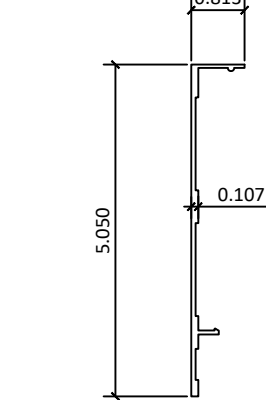
11 2800-25 – BOTTOM COVER
