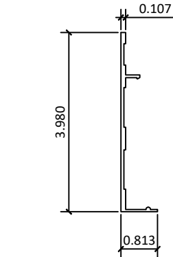
12 2800-26 – TOP COVER
